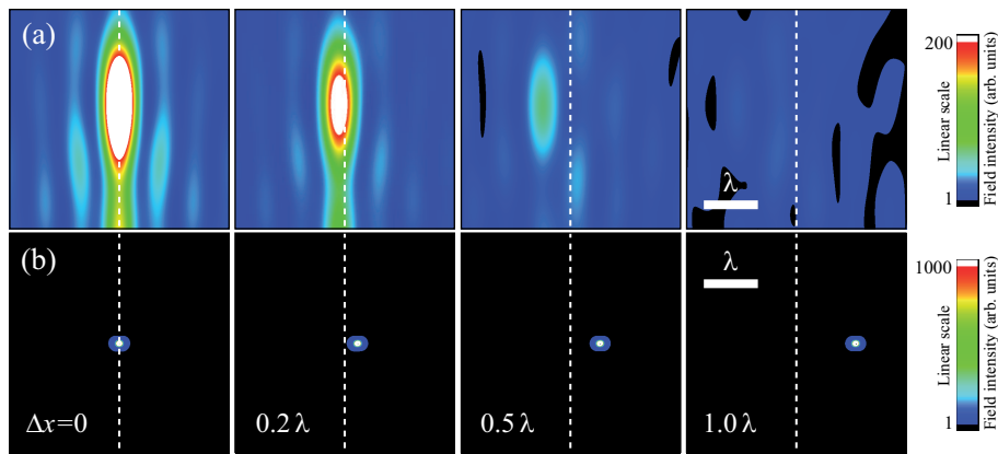
Fig. 6. Focusing of off-axis spots. The lower images (b) show different source spots, laterally displaced away from the axis of the lens by a distance \Delta x as indicated by labels. The upper images (a) show the corresponding image spots. The vertical dashed lines indicate the lens axis. The antenna has 30 silicon rings embedded in silica and a focal distance of 10\lambda . The free-space light wavelength is \lambda_0 = 1550 nm. The external dipole is like in Eq. (5).
